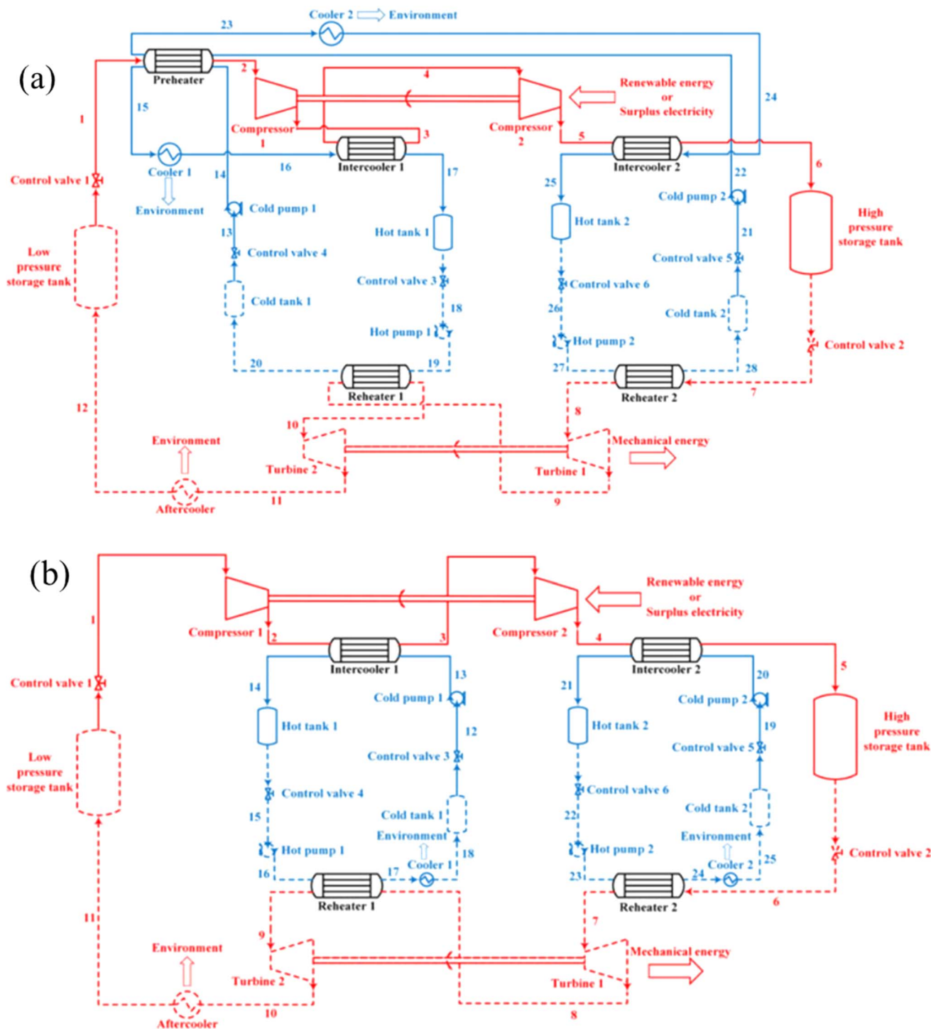
Fig. 8 (a) A carbon-dioxide energy storage system based on Brayton cycle; 59 (b) an ultra-carbon dioxide energy storage system based on Brayton cycle. 59
