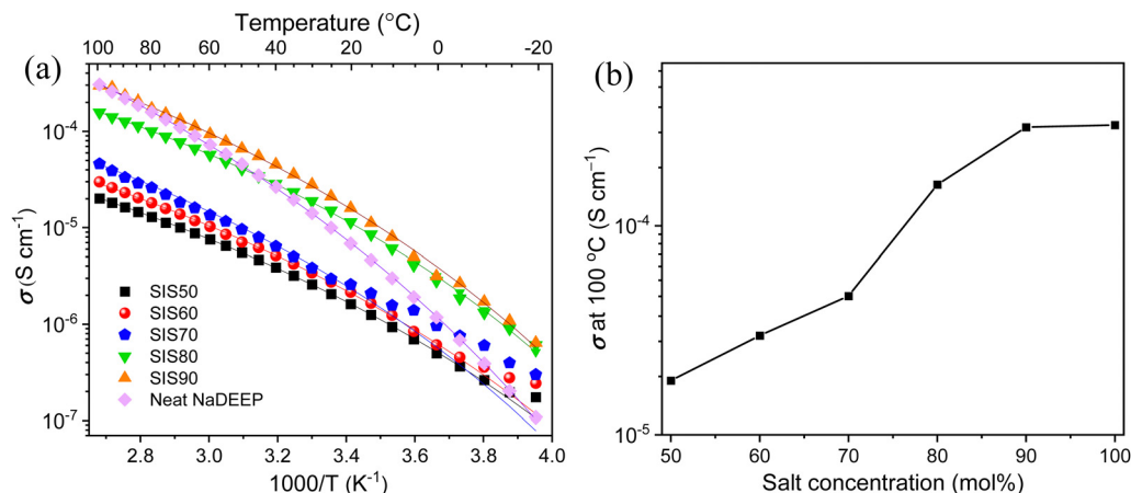
Fig. 3 Ionic conductivity as a function of (a) temperature for the neat NaDEEP salt and the SISXX electrolytes, and (b) salt concentration at 100 °C.
