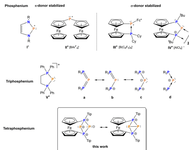
Fig. 1 Comparison of phosphenium ions \text{I}^+ , \text{II}^+ , 50 \text{III}^+ , 42 and \text{IV}^+ , 54 (top) to triphosphenium ions \text{V}^+ (middle) and a tetraphosphenium ion (bottom).
