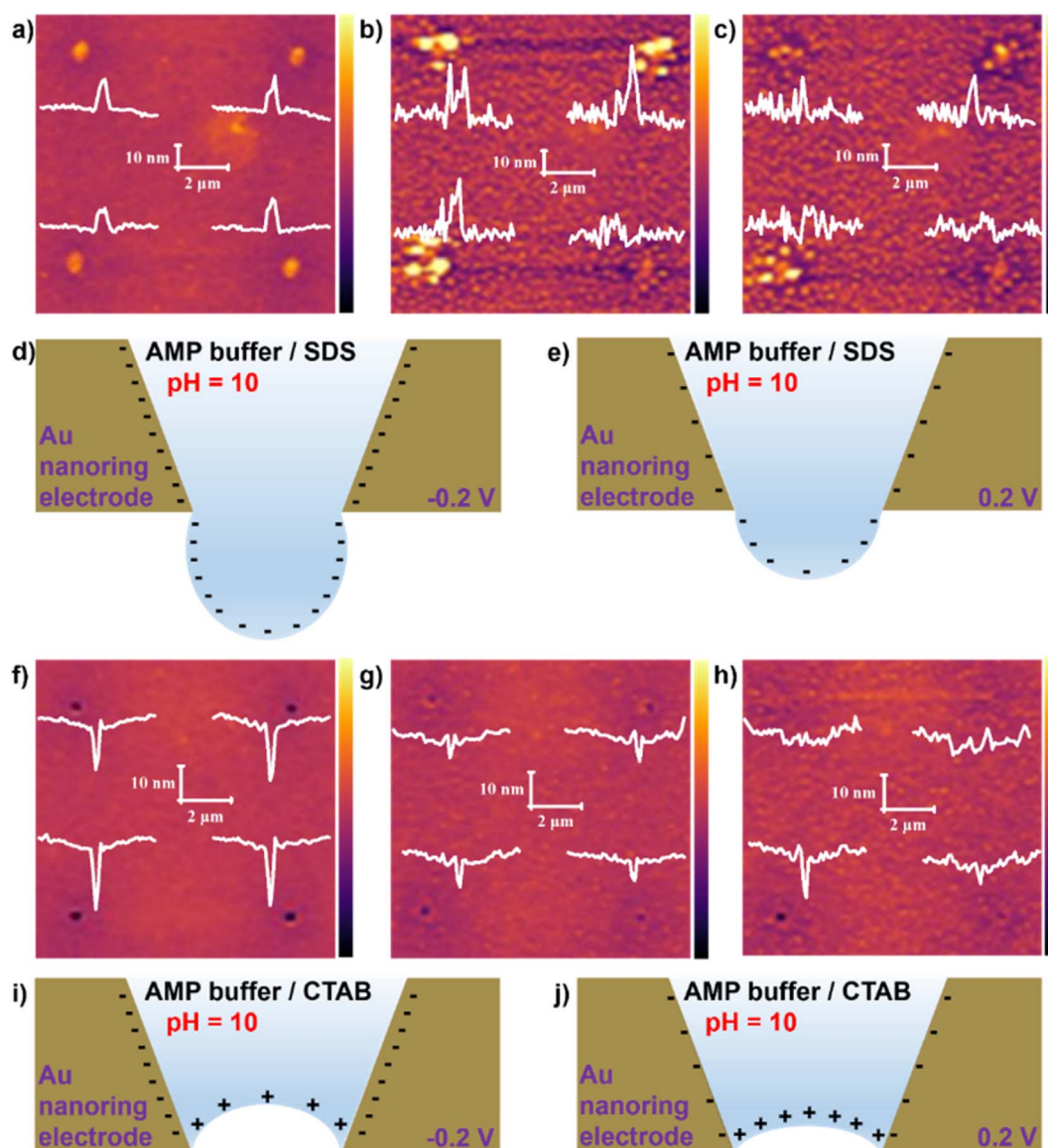
Fig. 3 AFM characterization of the effect of surfactants on the nanointerfaces curvature in AMP buffers. AFM characterization of the nano-interfaces after the addition of (a–c) 40 \mu\text{M} SDS at (a) no potential, (b) -0.2 V, and (c) 0.2 V, and (f–h) CTAB at (f) no potential, (g) -0.2 V, and (h) 0.2 V; the insets show the specific height of each nanodroplet. Schematic of nanointerfaces subjected to electrostatic forces from Au nanoring electrodes after the addition of (d and e) SDS at (d) -0.2 V and (e) 0.2 V and (i and j) CTAB at (i) -0.2 V and (j) 0.2 V.
