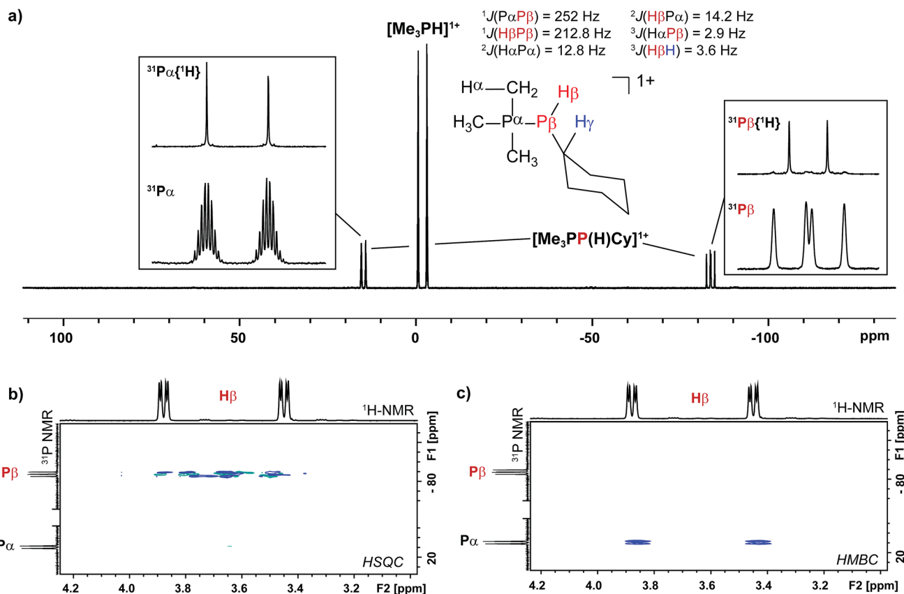
Fig. 5 (a) 31 P NMR spectrum of the crude reaction mixture containing CyPH 2 and [10(Me)][OTf] 4 in a 2 : 1 ratio. Insets show detailed views of the 31 P{ 1 H} and 31 P NMR resonances assigned to the Me 3 P- (left) and -P(H)Cy (right) fragments in [Me 3 PP(H)Cy] 1+ . A list of coupling constants deduced from the combination of 31 P and 1 H NMR is also given. (b) Sections of the 31 P/ 1 H HSQC spectrum showing a 1 J PH coupling between P β and H β . (c) Sections of the 31 P/ 1 H HMBC spectrum showing a 2 J PH coupling between P α and H β .
