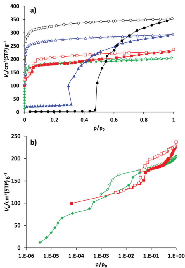
Fig. 5 Nitrogen physisorption isotherms for compounds 1' – 4' at 77 \text{ K} : (a) linear representation of the isotherms; (b) isotherms of compounds 3' and 4' on a semilogarithmic scale. Black circles – 1' , blue triangles – 2' , red squares – 3' , and green diamonds – 4' . Close symbols – adsorption, and open symbols – desorption.
