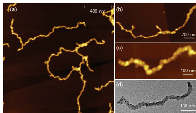
Fig. 5 AFM images of the nanostructures from \text{PPP(EH)-}b\text{-P3MT} s on HOPG: (a) \text{PPP(EH)}_{100}\text{-}b\text{-P3MT}_{90} . (b) \text{PPP(EH)}_{100}\text{-}b\text{-P3MT}_{130} . (c) High-resolution AFM images of the nanostructures from \text{PPP(EH)}_{100}\text{-}b\text{-P3MT}_{130} . (d) TEM images of the nanostructures from \text{PPP(EH)}_{100}\text{-}b\text{-P3MT}_{130} on a Cu/C TEM grid.
