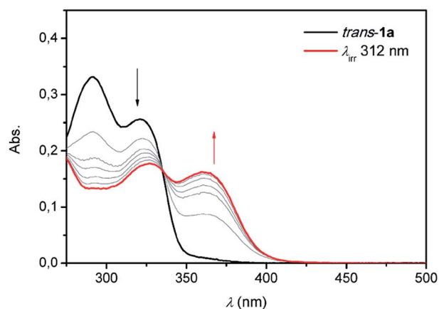
Fig. 2 UV-Vis spectral changes upon irradiation with 312 nm light starting with trans - 1a (black) at 1 \times 10^{-5}\text{ M} in DMSO and ending at the PSS (red).
