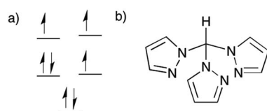
Fig. 1 (a) Scheme of the orbital splitting for 1 and 2 . (b) Tpm ligand.
