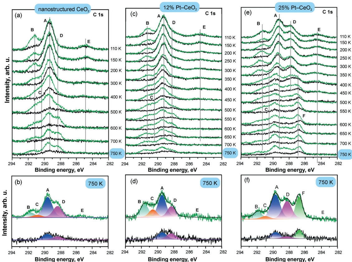
Fig. 18 C 1s spectra obtained from Pt-free nanostructured \text{CeO}_2 (a and b), 12% Pt- \text{CeO}_2 (c and d), and 25% Pt- \text{CeO}_2 (e and f) films prepared at 110 K on \text{CeO}_2(111)/\text{Cu}(111) annealed at different temperatures (black) and exposed to 50 L of CO at 110 K (green); the structure of the C 1s spectra obtained from Pt-free nanostructured \text{CeO}_2 (b), 12% Pt- \text{CeO}_2 (d), and 25% Pt- \text{CeO}_2 film (f) annealed to 750 K before (black) and after CO adsorption (green). The components labelled A–F arise from tridentate (A and C) and bidentate carbonates (B), carbonite (D), atomic carbon (E), and CO adsorption on metallic Pt particles (F). Adapted from ref. 112 with permission from the PCCP Owner Societies.
