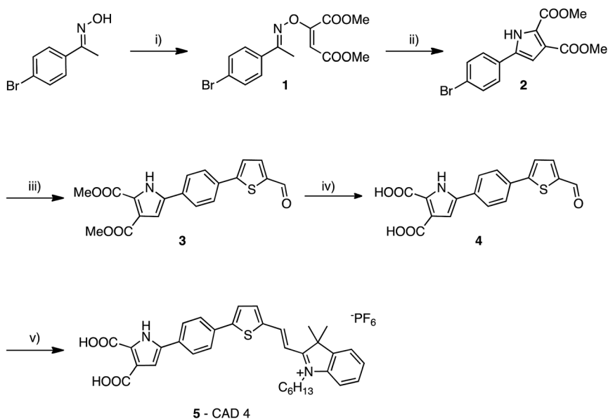
Fig. 2 Synthesis of CAD4. (i) DABCO, dimethyl acetylenedicarboxylate, DCM, -10^{\circ}\text{C} to rt, 17 h, 92%, (ii) toluene, microwave irradiation, 170 °C, 45 min, 74%, (iii) 5-formyl-2-thienylboronic acid, Pd(PPh 3 ) 2 Cl 2 , NaCO 3 , H 2 O/DME, 90 °C, 18 h, 87%, (iv) MeOH/H 2 O, NaOH, reflux, 12 h, 80%, (v) 1-hexyl-2,3,3-trimethyl-3H-indol-1-ium hexafluorophosphate, piperidine, MeCN, reflux, 48 h, 42%.
