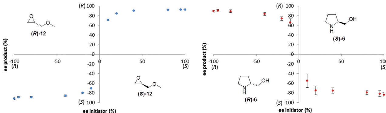
Fig. 3 Influence of enantiopurity of the triggering substance (at 20 mol%) on the enantiopurity of the Soai product, 2, formed in the reaction.
