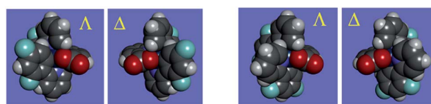
Fig. 1 Structures of FIRpic: \Lambda - and \Delta -enantiomers of mer - cis -C–C– trans -N–N isomer (left pair) and those of the mer - cis isomer (right pair) optimized by DFT calculations. Detailed conditions of calculations are found in ESI.†
