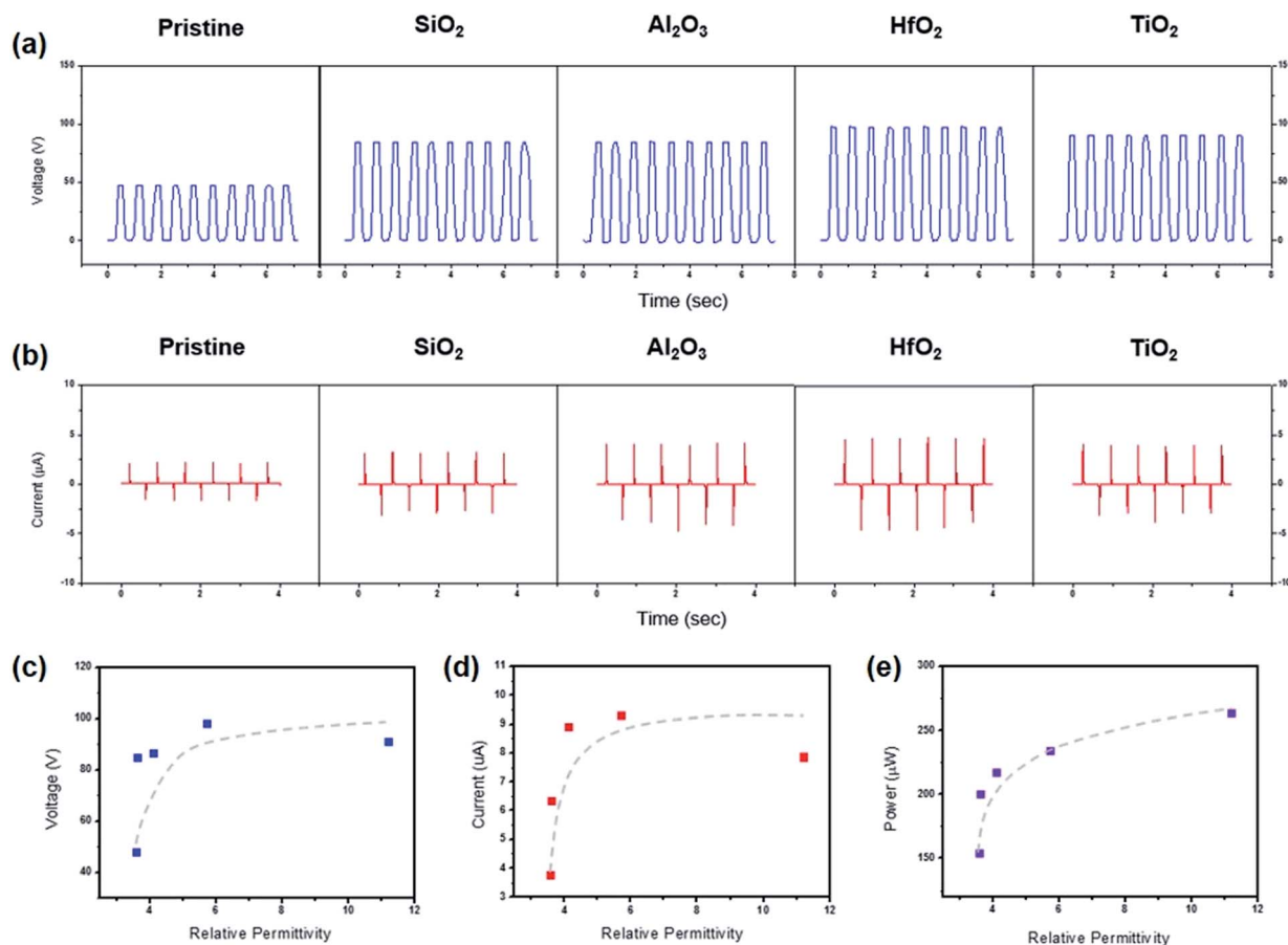
Fig. 5 Electrical data for the composite TENGs. (a) V_{\text{oc}} was measured using a Keithley 6514B electrometer. The output voltages for pristine PMMA and the composites consisting of \text{SiO}_2 , \text{Al}_2\text{O}_3 , \text{HfO}_2 and \text{TiO}_2 nanoparticles are, respectively, 47.5 V, 84.7 V, 86.3 V, 97.9 V and 90.7 V. (b) I_{\text{sc}} was measured using a Keithley 6485 picoammeter and a Tektronix DPO 2024 oscilloscope. The output currents for pristine PMMA and the composites consisting of \text{SiO}_2 , \text{Al}_2\text{O}_3 , \text{HfO}_2 and \text{TiO}_2 nanoparticles are, respectively, 3.76 \mu\text{A} , 6.32 \mu\text{A} , 8.88 \mu\text{A} , 9.28 \mu\text{A} and 8.16 \mu\text{A} . (c, d and e) V_{\text{oc}} , I_{\text{sc}} and power as a function of relative permittivity, respectively.
