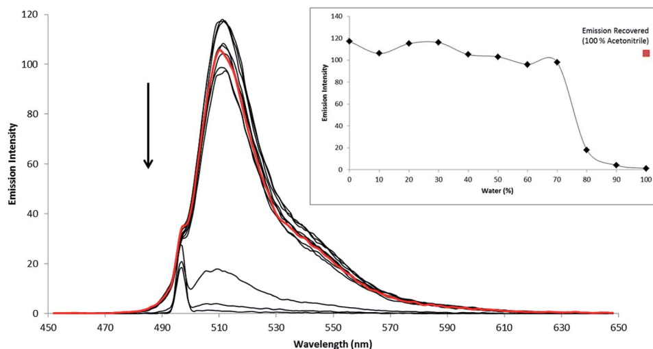
Fig. 3 Quenching of the fluorescent emission of compound 5 (10 \mu M) in acetonitrile–water solutions. The water ratio was varied from 0% to 98%. The red plot signifies the emission recovery of the BODIPY compound. (Inset) shows the changes to peak fluorescence intensity upon dilution by water and the corresponding emission recovery (red data point). The shoulder at 496 nm is artefactual due to the excitation source, 2.5 nm slit widths were used throughout.
