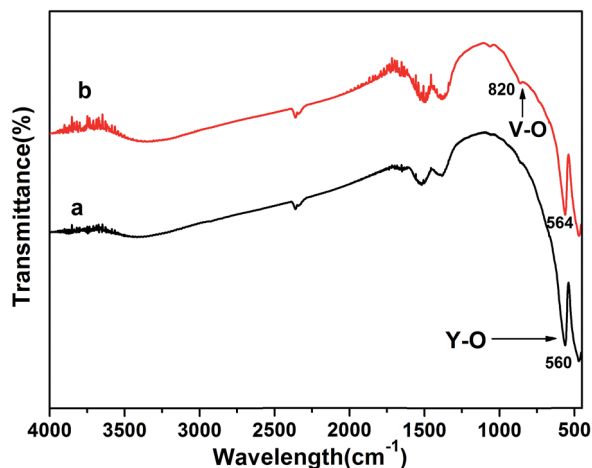
Fig. 2 FT-IR spectra of pure Y 2 O 3 :Eu 3+ (a) and rod-Y 2 O 3 :Eu 3+ @0.01YVO 4 :Eu 3+ (b).
