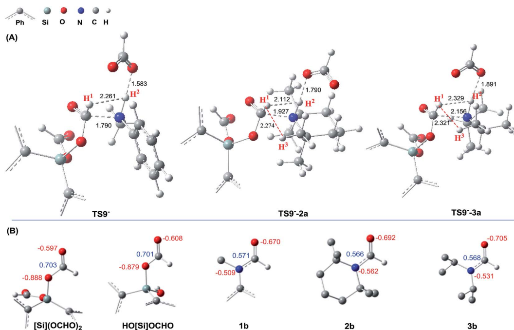
Fig. 6 (A) Comparing the structures of the transition states (TS9 - , TS9 - -2a, and TS9 - -3a) resulting in 1a, 2a, and 3a formylations. (B) Comparing the NBO charges (in e) of [\text{Si}](\text{OCHO})_2 and \text{HO}[\text{Si}]\text{OCHO} with those of formamides ( 1b–3b ).
