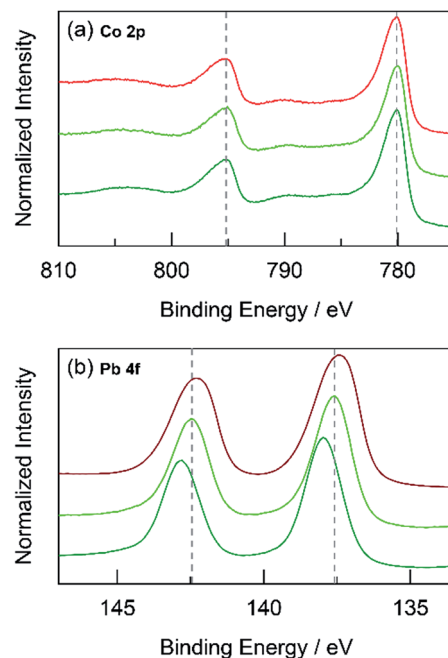
Fig. 11 High-resolution XPS spectra in the (a) Co 2p and (b) Pb 4f regions for: \text{CoPbO}_x (light green —) and \text{CoFePbO}_x (dark green —) compared to \text{CoO}_x (red —), and \text{PbO}_x (brown —). Grey dotted lines are presented as guides.
