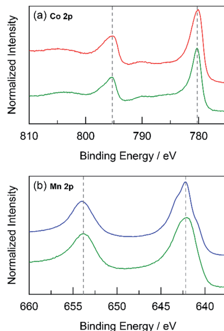
Fig. 10 High-resolution XPS spectra in the (a) Co 2p and (b) Mn 2p regions for: \text{CoMnO}_x (deposited at 0.90 V, dark green —) compared to \text{CoO}_x (red —), and \text{MnO}_x (blue —). Grey dotted lines are presented as guides.
