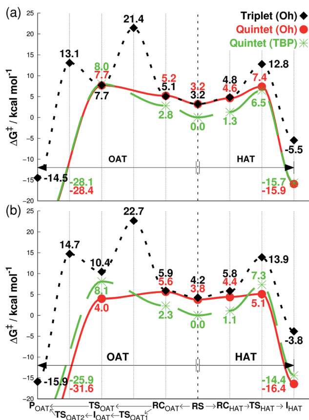
Fig. 2 Free energies calculated at 233 K ( \Delta G^\ddagger , see Methods section for details†), starting from separated reactants in the center of the graph and performing OAT (going left) or HAT (going right) for the oxidation of cyclohexene by Fe IV O complexes bearing (a) Me 3 NTB and (b) TQA ligands. The energy differences in the center between quintet (TBP) and other states correspond to the CH 3 CN binding energy as the sixth ligand. RS = reactants separated, RC = reactants complexed, TS = transition state, I = intermediate, P = product.
