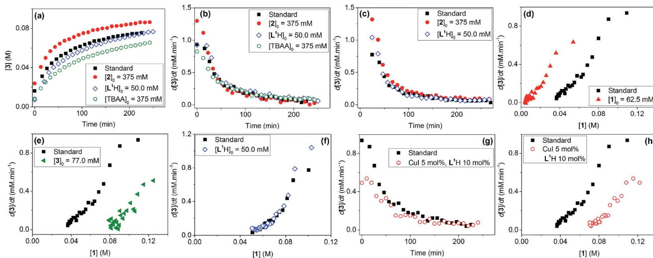
Fig. 1 Kinetic data for the reactions from 1 and 2 to 3 . Standard conditions: [1]_0 = 125.0 mM, [2]_0 = 187.5 mM, [L^1H]_0 = 25.0 mM, [CuI]_0 = 12.5 mM, [TBAH]_0 = 187.5 mM in d_7 -DMF. (a) [3] vs. time; (b) rate d[3]/dt vs. time; (c) rate d[3]/dt vs. time in d_3 -MeCN; (d) rate d[3]/dt vs. [1] in the 'same excess' experiments showing catalyst deactivation; (e) rate d[3]/dt vs. [1] showing product inhibition; (f) rate d[3]/dt vs. [1] showing the dependence of the reaction rate on catalyst loading; and (g) and (h) rate d[3]/dt vs. [1] showing the dependence of the reaction rate on catalyst loading.
