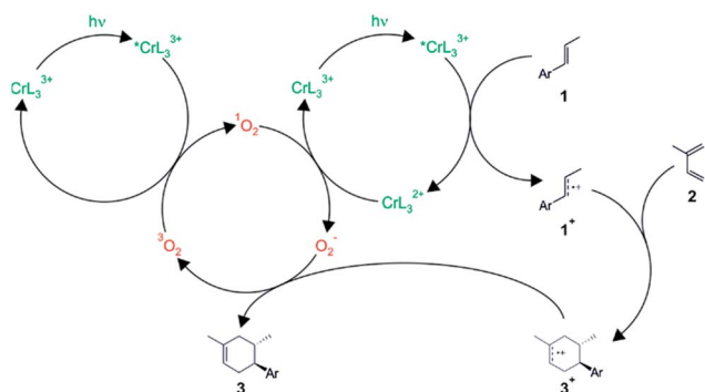
Fig. 5 Plausible mechanism for the light-driven [4 + 2] cycloaddition reaction between a dienophile (1) and a diene (2) catalyzed by the \text{Cr(L}^3)_3^{3+} complex in presence of oxygen. 16
