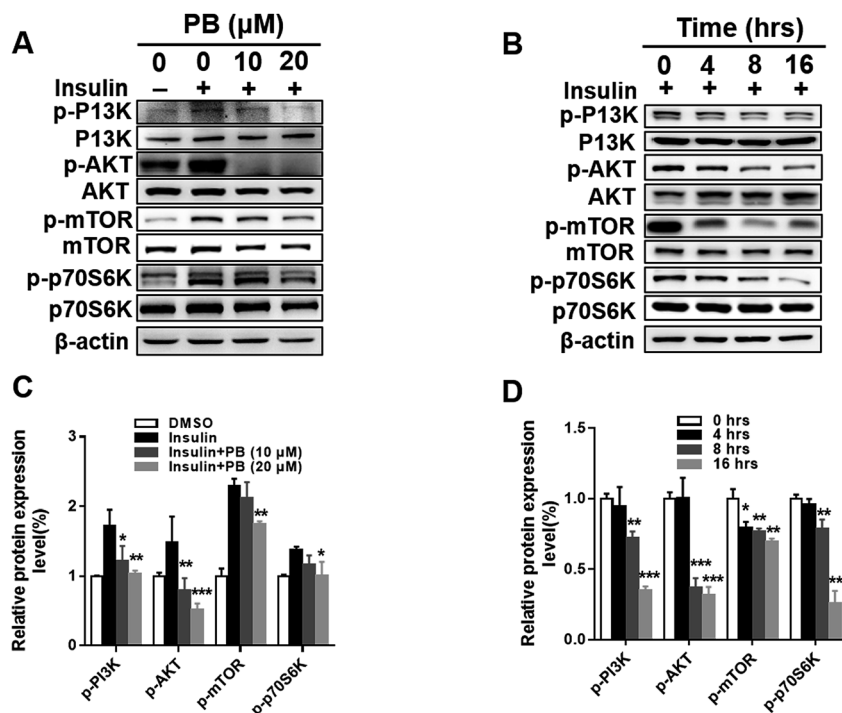
Fig. 2 Praeuptorin B inhibits the insulin induced PI3K/AKT/mTOR signaling pathway. HepG2 cells were pre-treated with insulin (100 nM) for 1 h and then treated the same concentration of insulin containing praeuptorin B indicated time periods (B) or increasing concentrations of praeuptorin B as indicated for 4 h (A). Whole cell extracts were subjected to WB with the antibodies as indicated. Statistical analysis. Expression of each protein was adjusted to actin as the loading control (C and D). All experiments were repeated three times. * p < 0.05 , ** p < 0.01 , *** p < 0.001 vs. DMSO.
