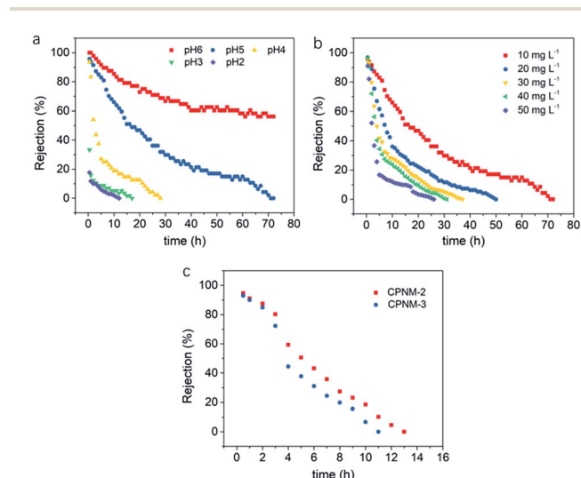
Fig. 8 Continuous filtration operation: (a) rejection rates of the CPNM-1 to Pb(II) aqueous solution under different pH environments (pH = 2–6; C_0 = 10 \text{ mg L}^{-1} ; 25^\circ \text{C} ); (b) rejection rates of the CPNM-1 to Pb(II) aqueous solution with different initial concentrations (pH = 5; C_0 = 10\text{--}50 \text{ mg L}^{-1} ; 25^\circ \text{C} ); (c) changes of rejection ratio of the CPNM-2 and CPNM-3 to Pb(II) aqueous solution with filtration time (pH = 5; C_0 = 10 \text{ mg L}^{-1} ; 25^\circ \text{C} ).
