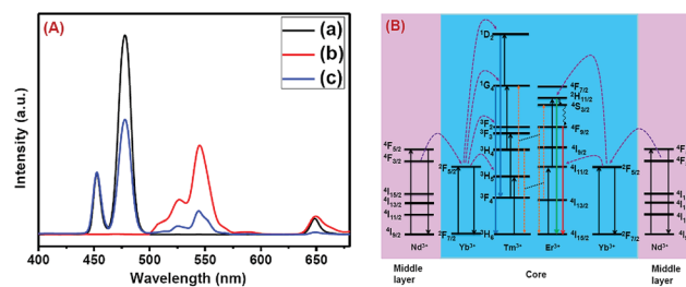
Fig. 6 (A) Comparison of UCL spectra of (a) \text{NaGdF}_4:\text{Tm}^{3+}(0.75)/\text{Yb}^{3+}(40)/\text{Nd}^{3+}(1)/\text{Ca}^{2+}(7)@\text{NaGdF}_4:\text{Ca}^{2+}(7)/\text{Nd}^{3+}(30) , (b) \text{NaGdF}_4:\text{Er}^{3+}(2)/\text{Yb}^{3+}(40)/\text{Nd}^{3+}(1)/\text{Ca}^{2+}(7)@\text{NaGdF}_4:\text{Ca}^{2+}(7)/\text{Nd}^{3+}(30) and (c) \text{NaGdF}_4:\text{Tm}^{3+}(0.75)/\text{Er}^{3+}(2)/\text{Yb}^{3+}(40)/\text{Nd}^{3+}(1)/\text{Ca}^{2+}(7)@\text{NaGdF}_4:\text{Ca}^{2+}(7)/\text{Nd}^{3+}(30) core/shell UCNPs, upon 808 nm laser excitation, to verify the cross-relaxation between \text{Tm}^{3+} and \text{Er}^{3+} ions. (B) Energy level diagram indicating the cross-relaxation mechanism between \text{Tm}^{3+} and \text{Er}^{3+} ions in \text{NaGdF}_4:\text{Tm}^{3+}(0.75)/\text{Er}^{3+}(2)/\text{Yb}^{3+}(40)/\text{Nd}^{3+}(1)/\text{Ca}^{2+}(7)@\text{NaGdF}_4:\text{Ca}^{2+}(7)/\text{Nd}^{3+}(30) core/shell UCNPs, upon 808 nm laser excitation.
