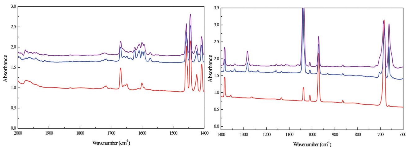
Fig. 2 Infrared spectra of the co-deposition of the samples of Ar/ cis -2-butene = 200 and Ar/ \text{O}_3 = 200. The blue line (middle) indicates initial deposition at 14 K and the purple line (top) represents the spectrum after annealing to 35 K, compared to a blank spectrum of Ar/ cis -2-butene = 200 (red, bottom).
