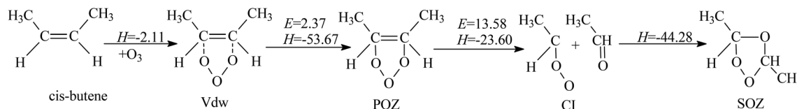
Fig. 1 The mechanism of cis -2-butene ozonolysis embedded with the energy barrier \Delta E and reaction energy \Delta H (all in kcal mol ^{-1} , 298.15 K). Geometries of the stationary points involved in the stabCI-OO + H _2 O reaction obtained at the M06-2x/6-311+G(d, p) level of theory. Bond lengths and intermolecular distances are given in Å.
