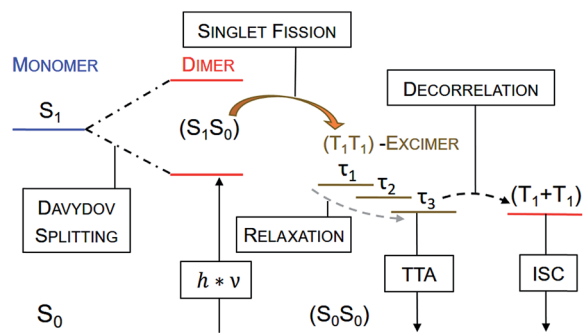
Fig. 11 Generalized mechanistic scheme illustrating all observed transitions and transient species at room temperature. No (T_1T_1) -excimer 3 was observed for dimers 4a – c . Triplet–triplet annihilation (TTA) is the main deactivation channel of the (T_1T_1) -excimer state for all dimers. Only dimer 4d shows a minor amount of free triplet, which is most likely generated by decorrelation and, therefore, termed as (T_1 + T_1) . The (S_1S_0) state is not directly observable at room temperature due to a too short lifetime, but its population is evidenced by measurements at cryogenic temperatures (see Fig. 6).
