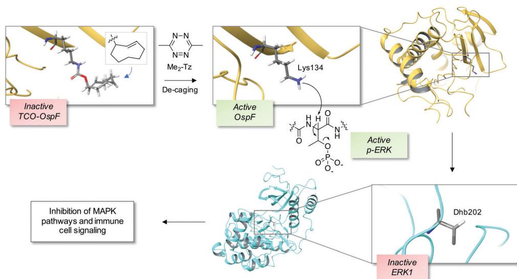
Fig. 2 A chemical de-caging strategy enabling control of the phospholyase activity of the bacterial enzyme OspF that irreversibly inactivates ERK1 via dehydrobutyrine (Dhb) formation. 23 A key step in the process is the use of the inverse electron demand Diels–Alder reaction to remove the TCO from the modified OspF to reveal the catalytic lysine that triggers phosphate elimination on p-ERK1 (OspF structure: PDB 3I0U; ERK1 structure: PDB 2ZOQ; TCO = trans -cyclooctene; Me 2 -Tz = 3,6-dimethyl-1,2,4,5-tetrazine).
