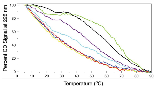
Fig. 3 Percent remaining CD signal at 228 nm as a function of temperature for the trpzp WT and mutant peptides. Line colors for all graphs: wild type, black; W2S, cyan; W4S, red; W9S, yellow; W11S, blue; K8L, purple; E5L, green. The curves represent the average of three independent determinations. The standard deviation for the percent of remaining CD signal between the three readings at any temperature was less than or equal to 2%.
