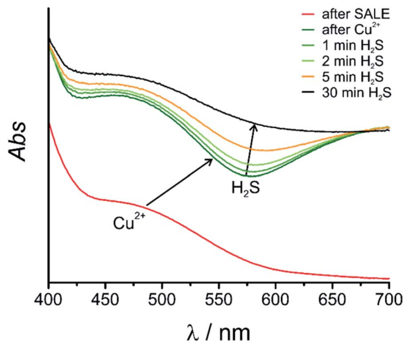
Fig. 2 UV/Vis spectra of the MIL-140D- sdc/abdc after the SALE with H 2 abdc (red), after the incorporation of \text{Cu}^{2+} (green) and after the exposure to 100 ppm \text{H}_2\text{S} with different time steps ranging from 1 to 30 minutes.
