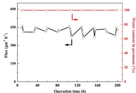
Fig. 15 Long-term operation evaluation of the SA-BS@GO-1.5 membrane.
