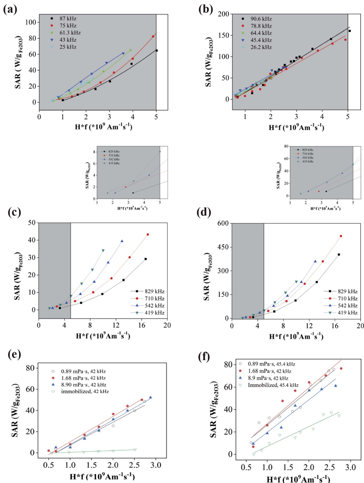
Fig. 4 SAR values in the low frequency range of aqueous suspension of (a) \epsilon -Fe 2 O 3 NPs and (b) \gamma -Fe 2 O 3 NPs as a function of health parameter Hf . SAR values in the high frequency range of aqueous suspensions of (c) \epsilon -Fe 2 O 3 NPs and (d) \gamma -Fe 2 O 3 NPs. In the insets, details of the SAR in the health safety range of Hf . Shaded areas mark the health safety region in a–d. SAR vs. Hf at different NP mobility conditions of (e) \epsilon -Fe 2 O 3 NPs and (f) \gamma -Fe 2 O 3 NPs.
