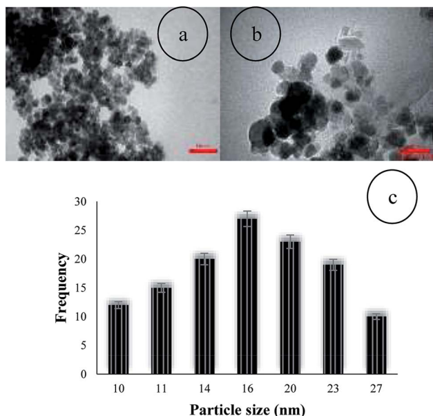
Fig. 7 TEM image (a and b) and particle size distribution histogram (c) of \text{Fe}_3\text{O}_4\text{@NFC@Co(II)} .
