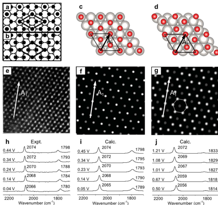
Fig. 1 Pt(111)(2 × 2)-3CO adstructures at 0.04–0.44 V vs. SHE in a CO-saturated 0.1 M HClO 4 aqueous solution: (a and b) the two possible adstructures (2 × 2)-3CO α 1 and α 2 , respectively, proposed by Villegas et al. ; (c and d) the respective optimized structures; (e) the measured EC-STM pattern; 44 (f and g) the corresponding calculated patterns of the α 1 and α 2 structures; (h) the measured EC-IR spectra; 47 and (i and j) the corresponding calculated spectra of the α 1 and α 2 adstructures. Images (a), (b) and (e) adapted from ref. 44 with permission, copyright (1994) American Institute of Physics; image (h) adapted from ref. 47 with permission, copyright (2000) American Chemical Society.
