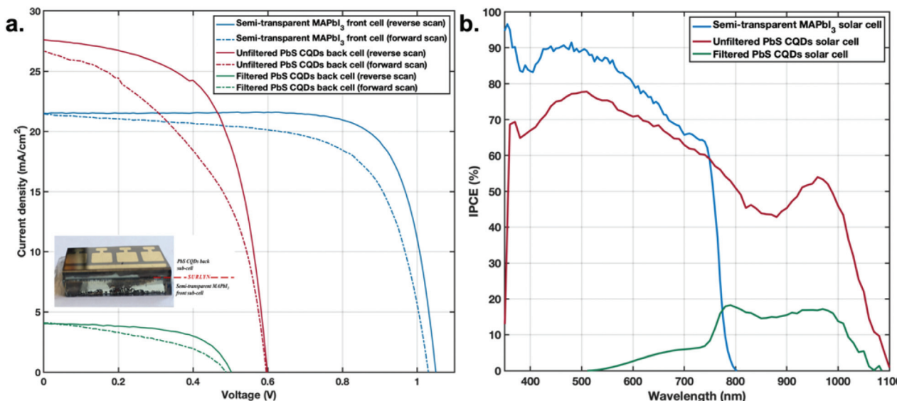
Fig. 3 Photovoltaic performance: (a) current–voltage ( J – V ) characteristics of unfiltered (red line) and filtered (green line) PbS CQD devices and the semi-transparent \text{MAPbI}_3 device (blue line), under illumination ( 1000 \text{ W m}^{-2} , AM 1.5G). The semi-transparent \text{MAPbI}_3 solar cell structure is as follows: FTO glass/compact \text{TiO}_2 /mesoporous \text{TiO}_2 / \text{MAPbI}_3 perovskite/Spiro-OMeTAD/10 nm Au/surlyn ( 25 \mu\text{m} ). The PbS CQD solar cell has the following configuration: indium doped tin oxide (ITO) glass/aluminum doped zinc oxide layer ( \text{AlZnO} )/PbS– \text{PbX}_2 ( \text{X} -halogen molecule)/PbS–EDT (EDT–1,2-ethanedithiol)/80 nm Au. PbS CQDs of \lambda_{\text{max}} = 935 \text{ nm} were used for these measurements. The filtered PbS CQD cell means that during the measurement, the semi-transparent \text{MAPbI}_3 solar cell was placed above the CQD cell – see the included profile picture of the perovskite–CQD tandem solar cell ( 2.4 \times 1.4 \text{ cm} in size). (b) IPCE spectra of the PbS CQD cell (red line), the \text{MAPbI}_3 perovskite cell with a 10 nm semi-transparent Au electrode (blue line) and the filtered PbS CQD cell with a semi-transparent \text{MAPbI}_3 cell as the filter (green line).
