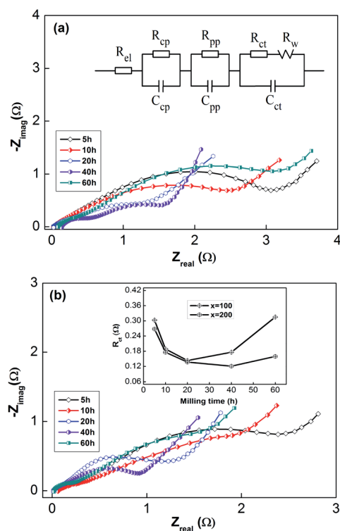
Fig. 6 Electrochemical impedance spectra (EIS) of as-milled \text{NdMg}_{11}\text{Ni} + x \text{ wt\% Ni} ( x = 100, 200 ) alloys: (a) x = 100 , (b) x = 200 .
