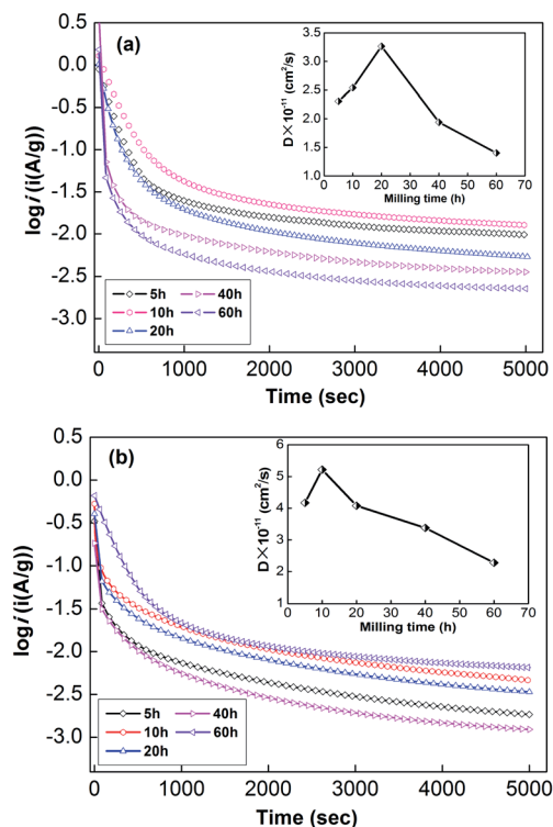
Fig. 5 Semilogarithmic curves of anodic current vs. time responses of as-milled \text{NdMg}_{11}\text{Ni} + x \text{ wt\% Ni} ( x = 100, 200 ) alloys: (a) x = 100 , (b) x = 200 .
