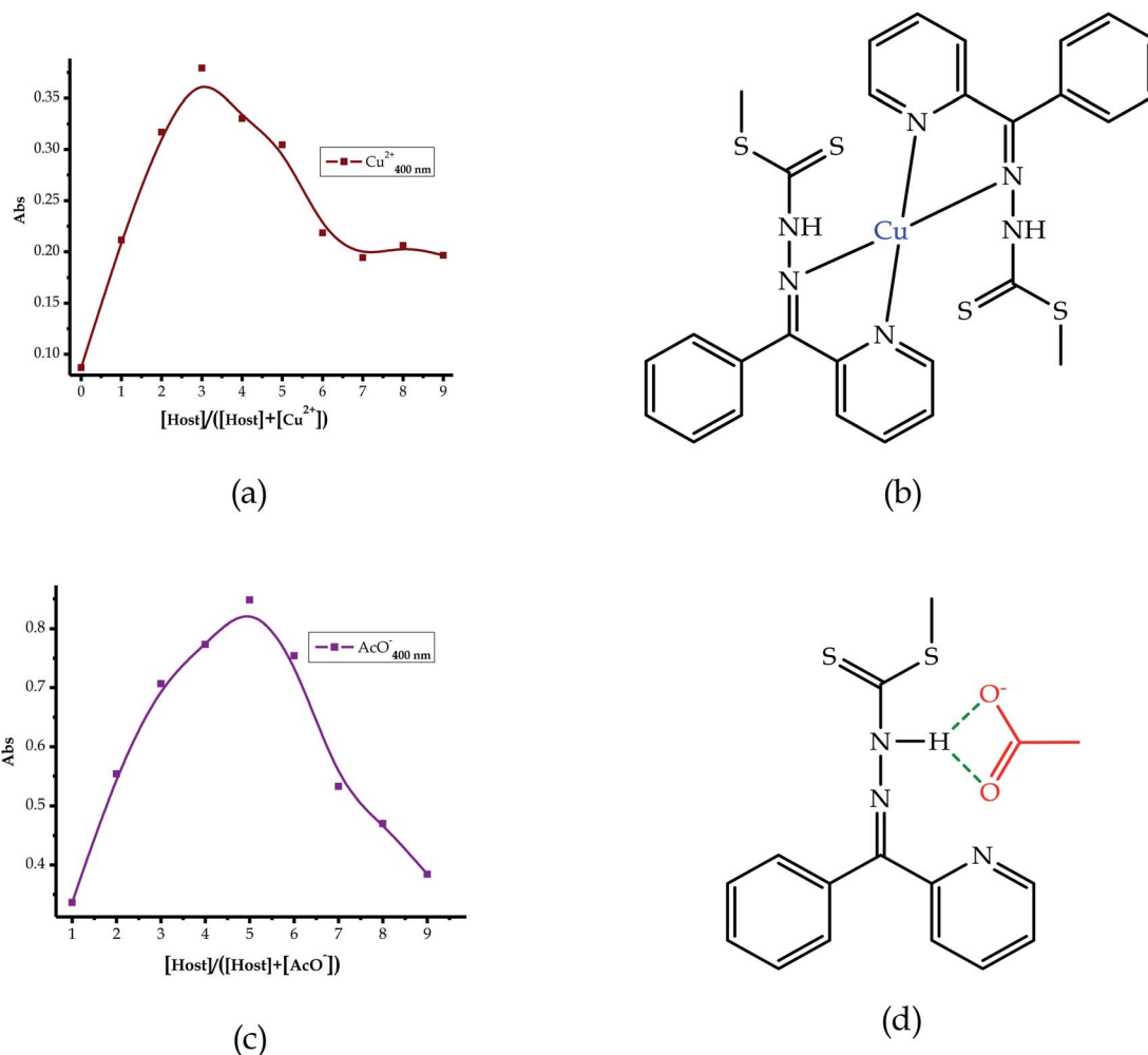
Fig. 7 The proposed interaction and binding modes of EN with the cations: (a) Job plot and (b) \text{EN-Cu}^{2+} , and anions: (c) Job plot and (d) \text{EN-AcO}^- .
