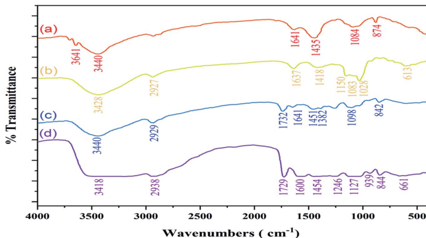
Fig. 4 Demonstration of comparative FT-IR spectra of (a) chitosan, (b) sodium alginate, (c) polyvinyl alcohol, (d) CS/PVA/SA hydrogels (without Ag 2 O/SiO 2 NPs and curcumin).
