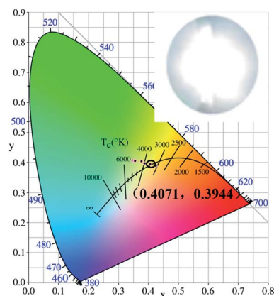
Fig. 16 Color coordinates of MYAS:0.05Dy 3+ ,yEu 3+ ( y = 0-0.1 ), and the warm white LED device (MYAS:0.05Dy 3+ ,0.07Eu 3+ + 370 nm UV LED chip) under a voltage of 3.2 V and current of 5 mA (CIE = (0.4071, 0.3944), CCT = 3500 K, CRI = 91.3).
