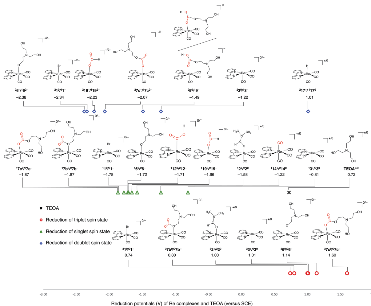
Fig. 3 One-electron reduction potentials (V vs. SCE) that were calculated for the triplet, singlet, and doublet spin states of the Re complexes. The label, 31^0/21^- , indicates that species 1 with zero charge in the triplet spin state is reduced to species 2 with minus one charge in the doublet spin state. The higher the positive value, the stronger the oxidizing power.
