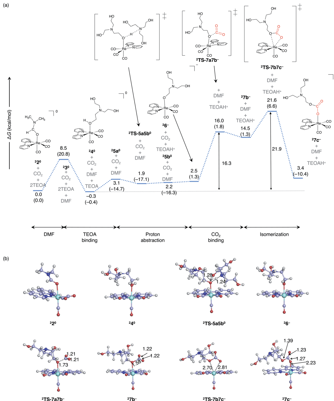
Fig. 6 (a) The free energy profile for the formation of the monoalkyl carbonate complex starting from the one-electron-reduced complex. \Delta G and \Delta H (in parentheses) are given in kcal mol ^{-1} . (b) Optimized key stationary points with the selected bond distances (Å). The blue bars represent one-electron-reduced doublet Re complexes.
