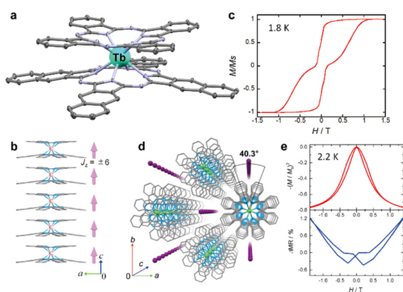
Fig. 24 (a) Crystal structure of [(\text{Nc})\text{Tb}(\text{Pc})]^+\text{PF}_6^- (CCDC YICQIN). Hydrogen atoms and the \text{PF}_6^- anion are omitted for clarity. (b) 1D structure of [(\text{Nc})\text{Tb}(\text{Pc})]^+\text{PF}_6^- along the c -axis. (c) MH measurement hysteresis loop with a coercivity ( H_C ) of 150 mT (1500 Oe) for a single crystal of [(\text{Nc})\text{Tb}(\text{Pc})]^+\text{PF}_6^- at 1.8 K ( H//c -axis). The data were normalized to the value in a field of 7 T. (d) 1D structure of [\text{Dy}(\text{Pc})_2]\text{I}_x along the c -axis. Hydrogen atoms are omitted for clarity. (e) MH curve of [\text{Dy}(\text{Pc})_2]\text{I}_x for a polycrystalline sample at 2.2 K (top). Magnetoresistance (MR) measurement of [\text{Dy}(\text{Pc})_2]\text{I}_x for a single crystal at 2.2 K. Adapted with permission from (a–c) ref. 136 and (d and e) ref. 348. Copyright 2018 and Copyright 2021, Wiley-VCH.
