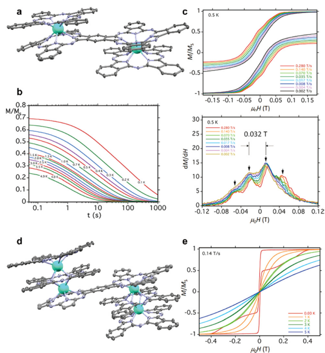
Fig. 23 Crystal structure of (a) (Pc)Ln(f-Pc 2 )Ln(Pc) OBu (Ln 3+ = Dy and Tb) and (d) (Pc) 2 Ln 2 (f-Pc 2 )Ln 2 (Pc) 2 OBu (Ln 3+ = Tb and Dy) and the micro-SQUID-measurement magnetization decay curves (b) and hysteresis loops for oriented crystalline samples of (c) (Pc)Tb(f-Pc 2 )Tb(Pc) OBu and (e) (Pc) 2 Dy 2 (f-Pc 2 )Dy 2 (Pc) 2 OBu . Molecular structures of (a) and (d) based on the cif files from ref. 217 and 220. Protons and n -butoxy groups in (Pc)Ln(f-Pc 2 )Ln(Pc) OBu and (Pc) 2 Ln 2 (f-Pc 2 )Ln 2 (Pc) 2 OBu are omitted for clarity. Adapted with permission from (a and b) ref. 217. Copyright 2018, American Chemical Society. Adapted with permission from (d and e) ref. 220. Copyright 2018, Wiley-VCH.
