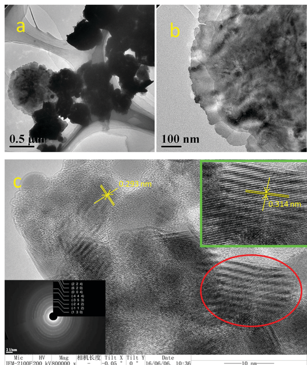
Fig. 3 TEM images of BiVO 4 at (a) 500 nm, (b) 100 nm scale magnifications, (c) high resolution TEM images and the corresponding lattice fringes at 10 nm scale with the SAED pattern.
