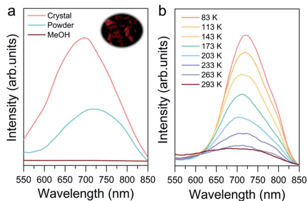
Fig. 6 (a) Emission spectra of crystals (pink line), powder (cyan line) and CH 3 OH solution (brown line) of Au8c . Inset: photograph of Au8c crystals under green light excitation. (b) Temperature-dependent emission spectra of Au8c in the crystalline state ( \lambda_{\text{ex}} = 365 nm).
