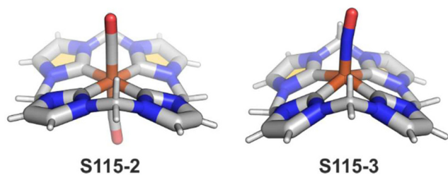
Fig. 26 Iron tetracarbenes complexes with calix[4]imidazolium.
