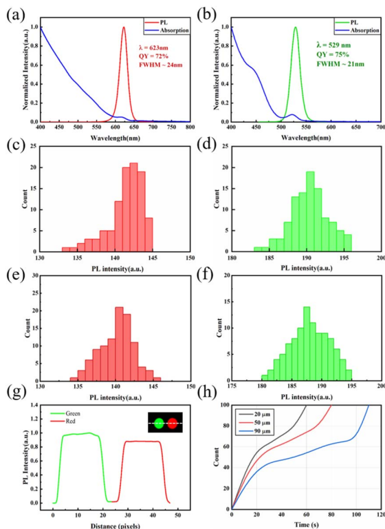
Fig. 4 Spectral curves of (a) red and (b) green CdSe/ZnS QDs. Histogram of average fluorescence intensity distribution with 10 \times 10 pixels of 50 \mu\text{m} (c) red and (d) green QDCCCLs, and 20 \mu\text{m} (e) red and (f) green QDCCCLs. (g) Fluorescence intensity of two adjacent red and green QD pixels in a dual-color QDCCCL with a pixel size of 20 \mu\text{m} . (h) Injection time of a monochrome QDCCCL with three different pixel sizes.
