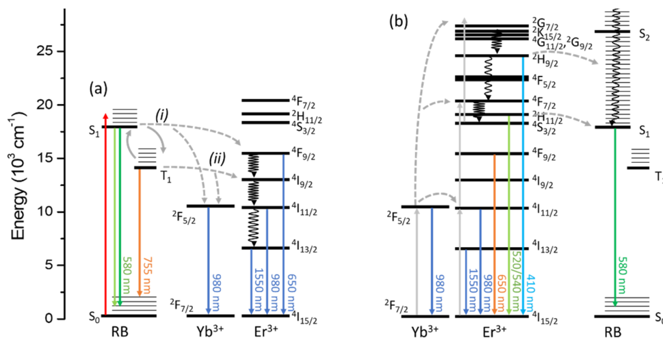
Fig. 1 Energy diagram of photophysical processes observed for UC Er @RB under N 2 exciting the (a) dye (λ exc = 560 nm) or the (b) UCNP (λ exc = 980 nm).
