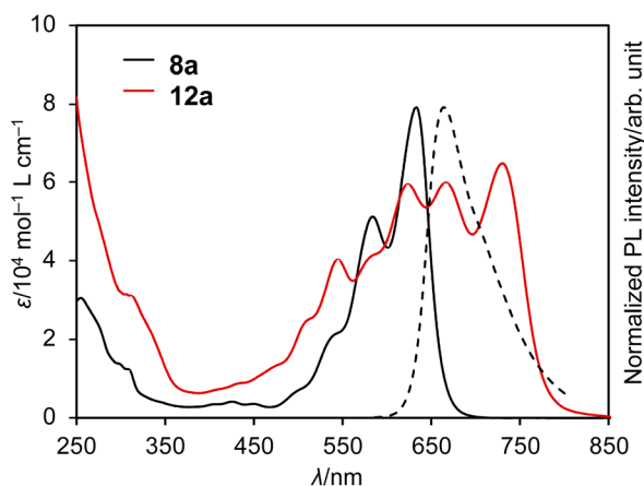
Fig. 5 UV/vis absorption spectra of 8a and 12a (solid lines) and emission spectrum of 8a (dashed line); solvent: CH 2 Cl 2 ; λ: wavelength; ε: extinction coefficient; λ ex = 550 nm.
