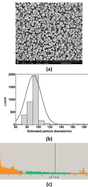
Fig. 3 Morphological study of electrodeposited nAuPt on the surface of GCE: (a) – SEM image; (b) – the particle size distribution of NPs electrodeposited on GCE, and (c) – X-ray spectral microanalysis.
