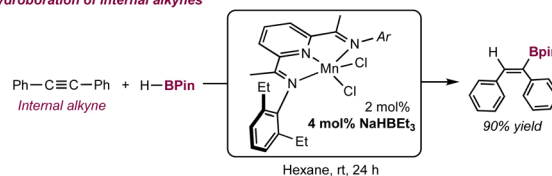
(b) This work: Activator-enhanced chemoselectivity for hydroboration
