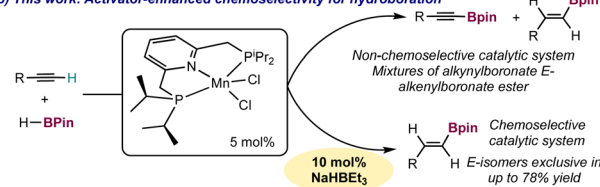
(b) This work: Activator-enhanced chemoselectivity for hydroboration
