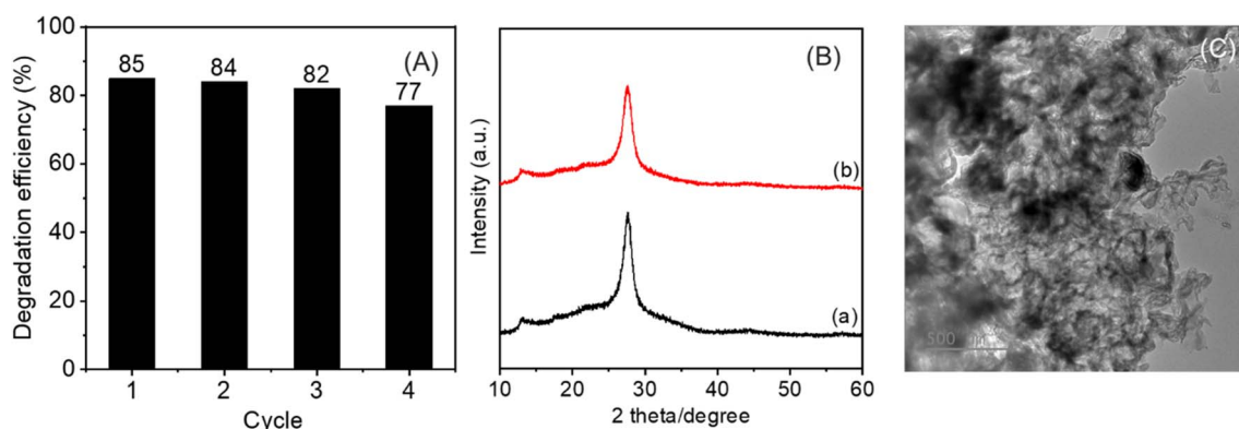
Fig. 9 Recycling of photocatalyst (A) of SMX upon the 3MnCN photocatalyst. XRD pattern (B) of 3MnCN of fresh (a) and reuse (b) and TEM image (C) of 3MnCN reuse.
