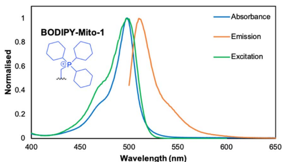
Fig. 2 Absorption (blue), emission (orange) and excitation (green) spectra of BODIPY-Mito-1 . [BODIPY] = 10 μM, PBS (pH = 7.4), 298 K. \lambda_{\text{ex}} = 497 nm, \lambda_{\text{em}} = 511 nm.
